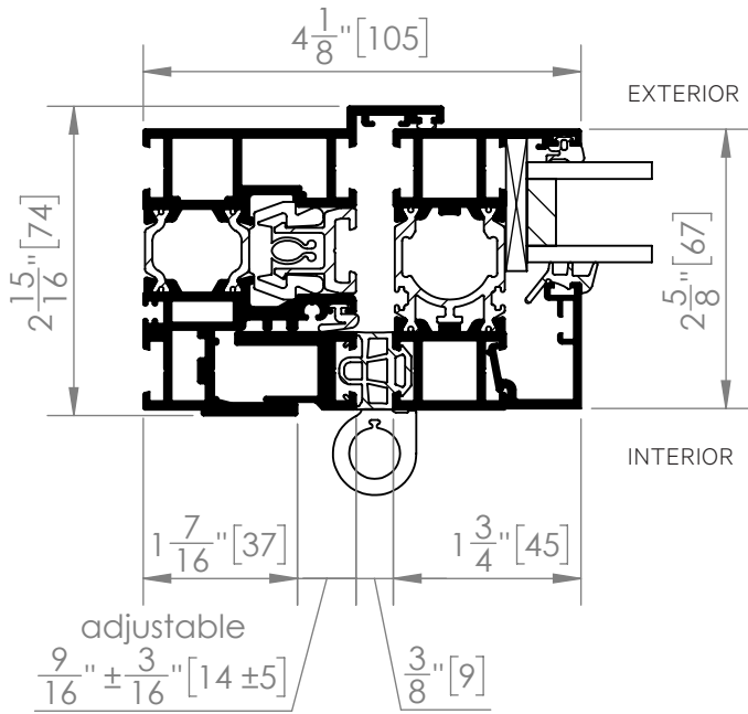
Detail 3.0 Panel Hinged to Side Jamb
