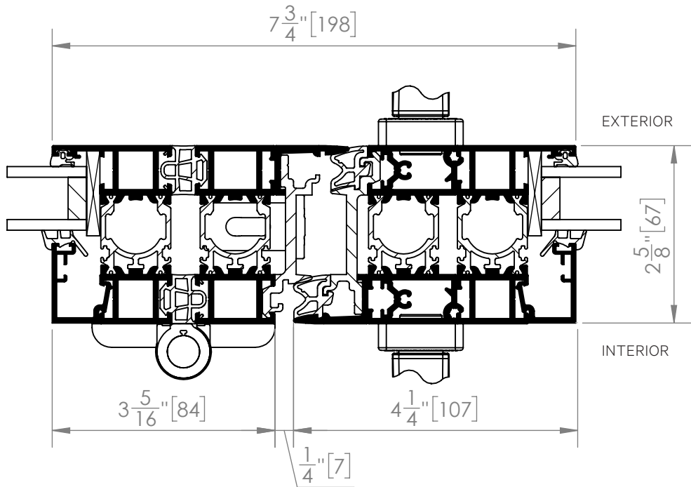
Detail 10.0 Meeting of Swing Panel with Locking and Folding Panel with Running Post and Top and Bottom Rollers Attached (Note: Daylight opening "DLO" of the panel with the running post will be 15/16" [33.5 mm] wider than the adjacent attached panel.)
