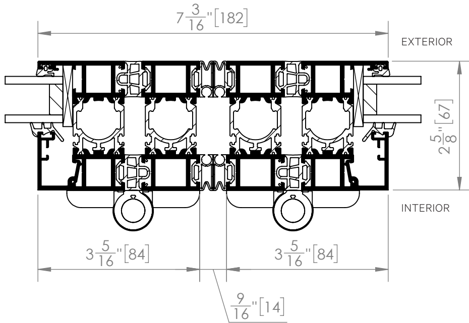
Detail 9.0 Meeting of Folding Panels with Running Post and Top and Bottom Rollers Attached (Note: Daylight opening "DLO" of the panels will be 15/16" [33.5 mm] wider than the adjacent attached panels.)
