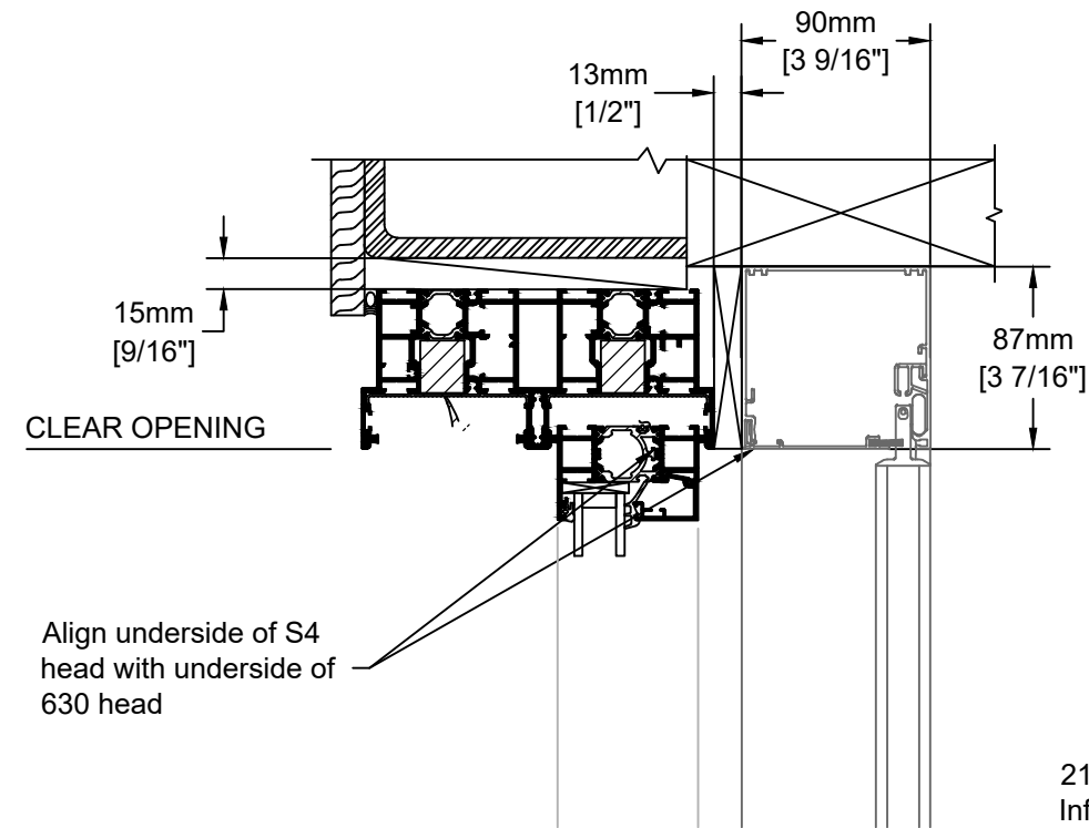
Vertical Section - Head
