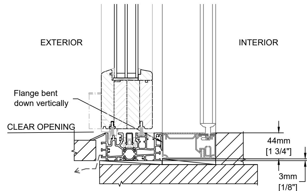
Vertical Section - Sill
