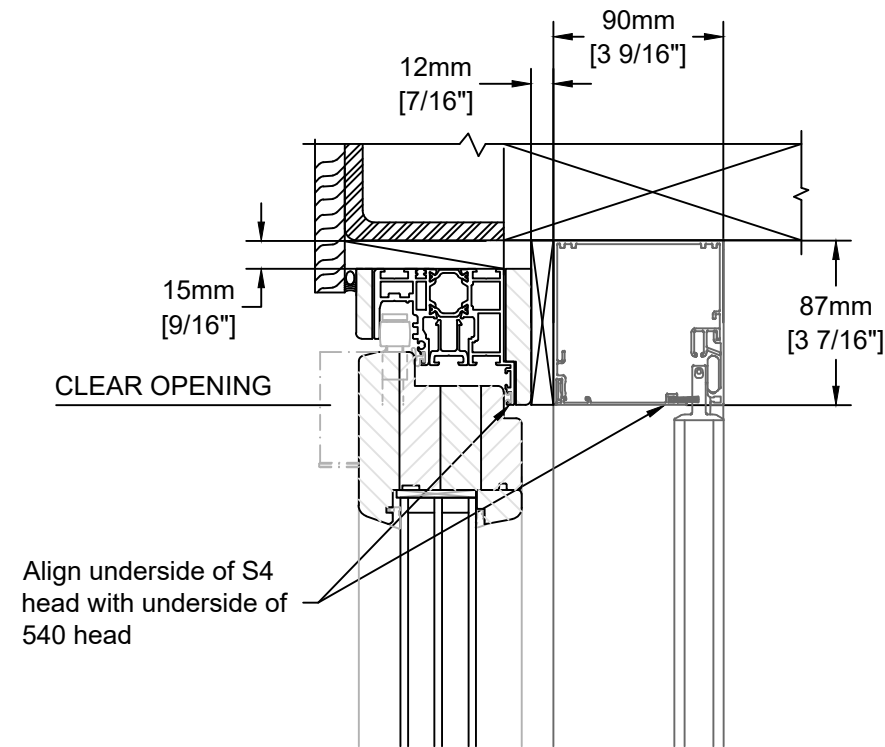
Vertical Section - Head
