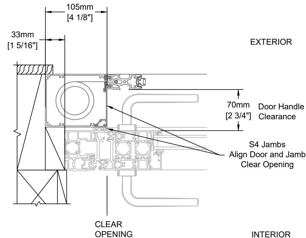
Horizontal Section Jamb with Handle
