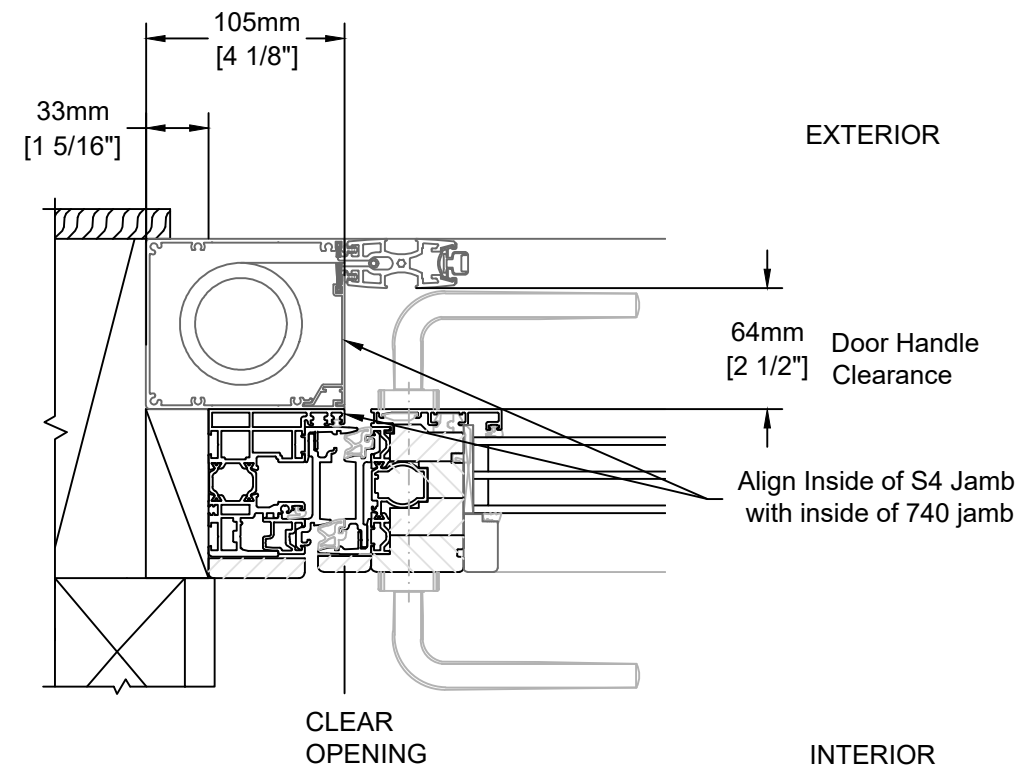
Horizontal Section Jamb with Handle
