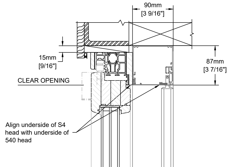
Vertical Section - Head
