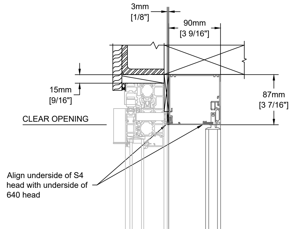
Vertical Section - Head
