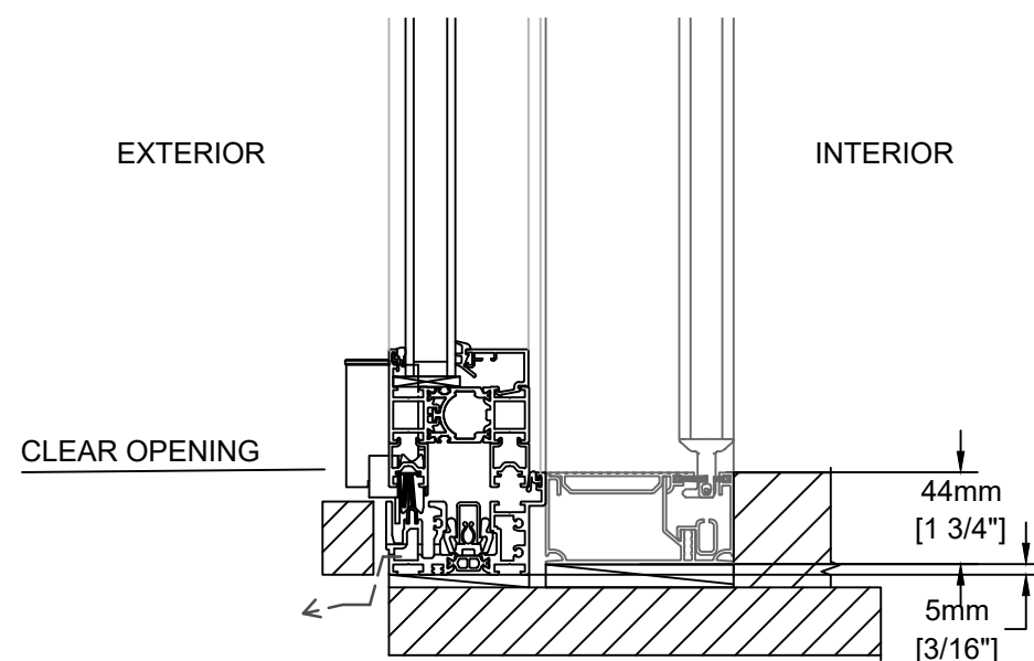
Vertical Section - Sill
