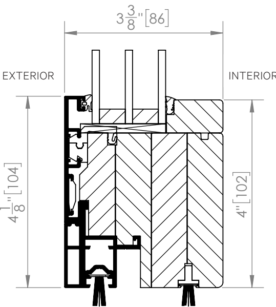
Typical Glass Stop Profile with Triple Glazing
