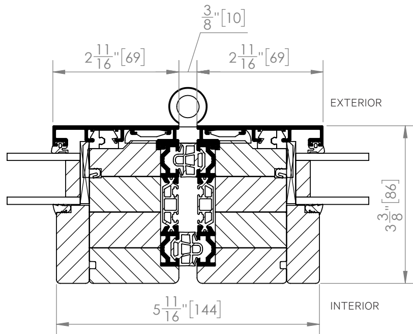
Detail 7C.1 Hinged Folding Panels
