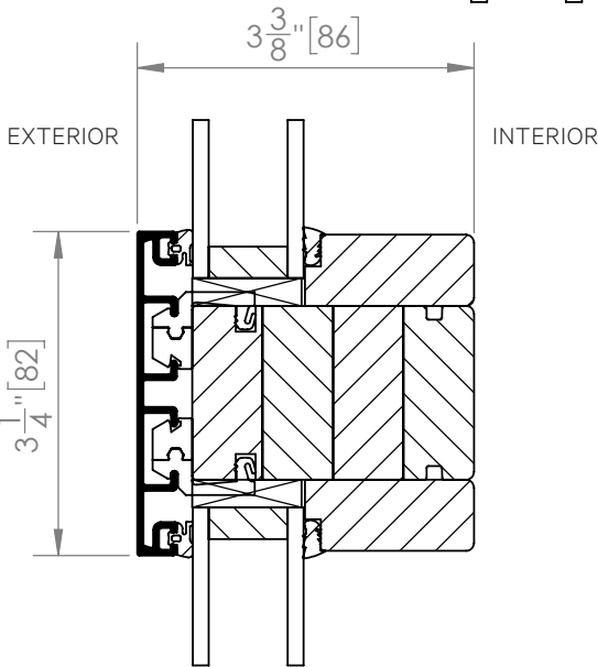
Typical Mullion Profile
