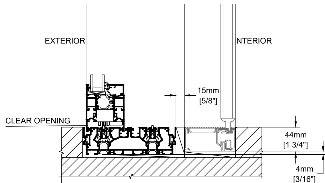
Vertical Section - Sill
