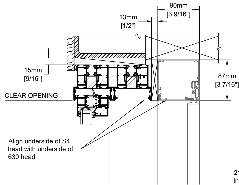
Vertical Section - Head
