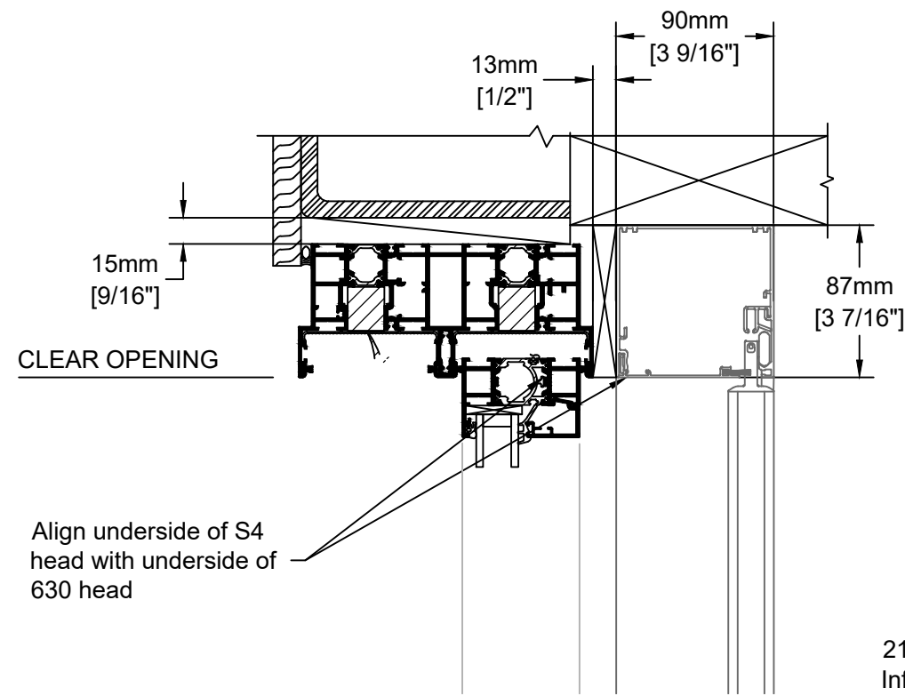
Vertical Section - Head
