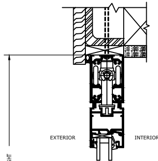
Head Track
