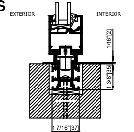
Flush Sill (Interior applications only)
