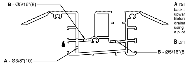
Low Profile Saddle Sill Option 1 Detail Drawing
