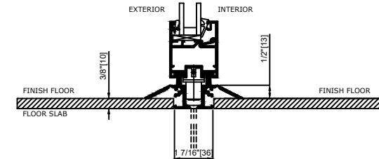
Interior Surface Mounted Sill - Option 1 (Interior applications only)
