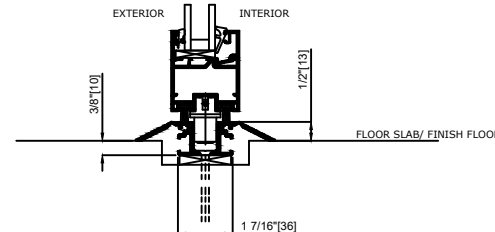
Interior Surface Mounted Sill - Option 2 (Interior applications only)
