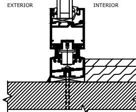
Standard Sill
