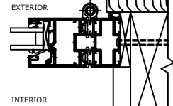
Panel Hinged at Right Side Jamb
