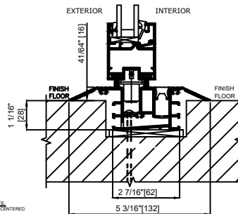
Low Profile Saddle Sill Option 1 Detail Drawing
