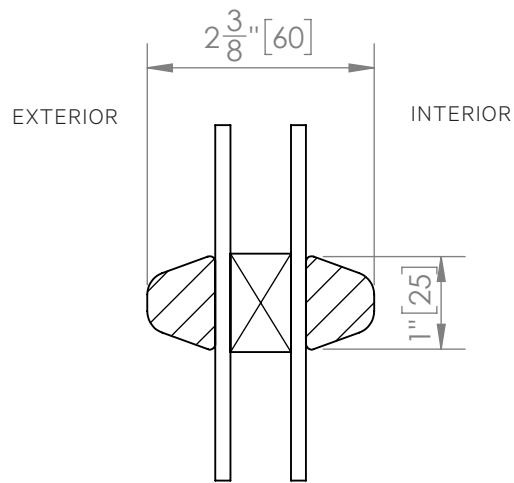
Typical Simulated Divided Lites with Spacer Bar
