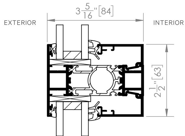
Typical Mullion Profile
