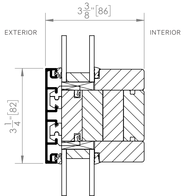
Typical Mullion Profile
