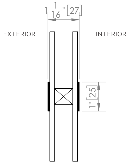
Typical Simulated Divided Lites with Spacer Bar
