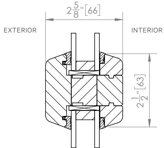
Typical Mullion Profile
